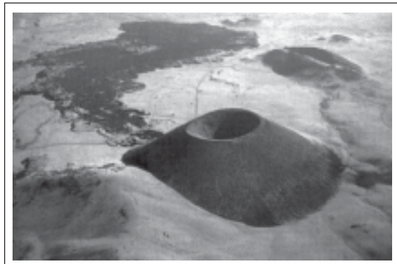
Shield Volcano
