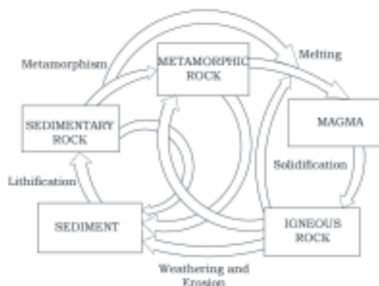
Fig 5.1 : Rock Cycle
