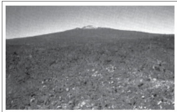
Cinder Cone
