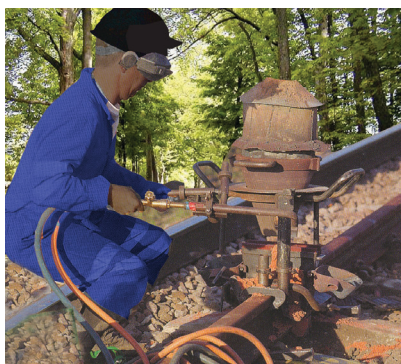
Figure 3.11 Thermit process for joining railway tracks
