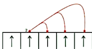
3 exchange by electron 2
