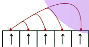
4 exchange by electron 1
