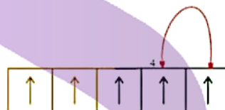
1 exchange by electron 4
