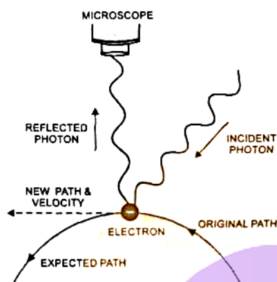
Change of momentum and position of electron on impact with a photon
