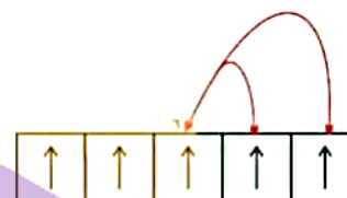
2 exchange by electron 3
