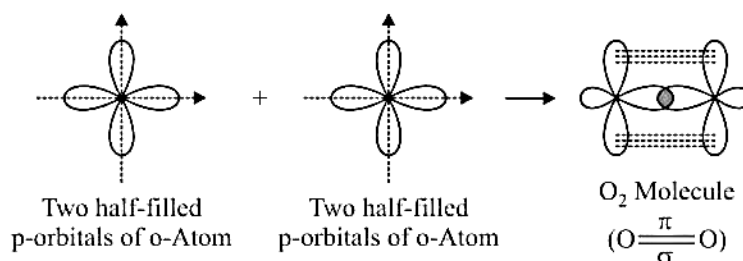
Formation of oxygen molecule
