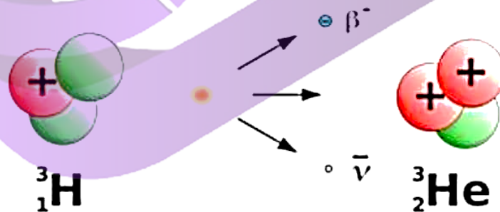
B-decay of a nucleus.
